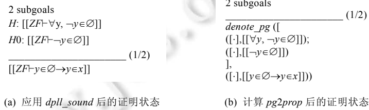
图 6 proof_goal 转换
