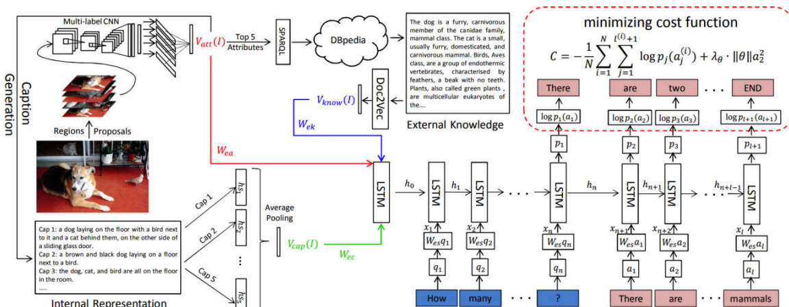
Fig.9 A VQA model with external knowledge [76]
