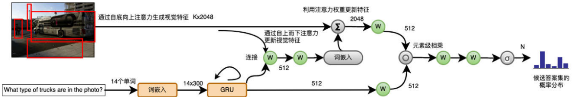
Fig.6 The overview of Bottom-Up and Top-Down Attention Model
