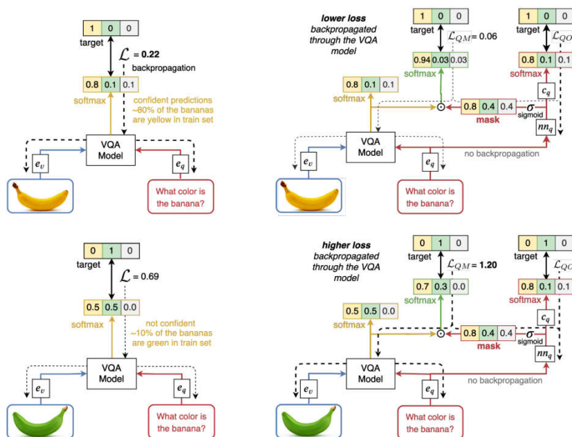
Fig. 10 Detailed illustration of the RUBi impact on the learning [85]
