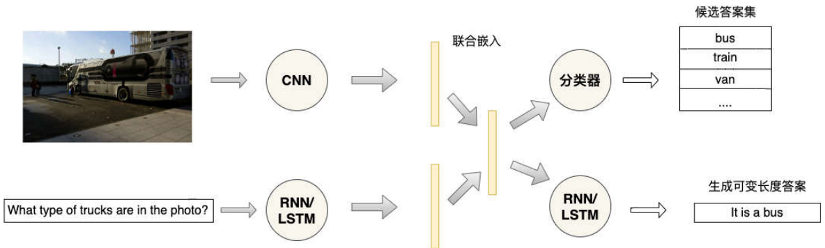
Fig.2 The framework of joint embedding methods
