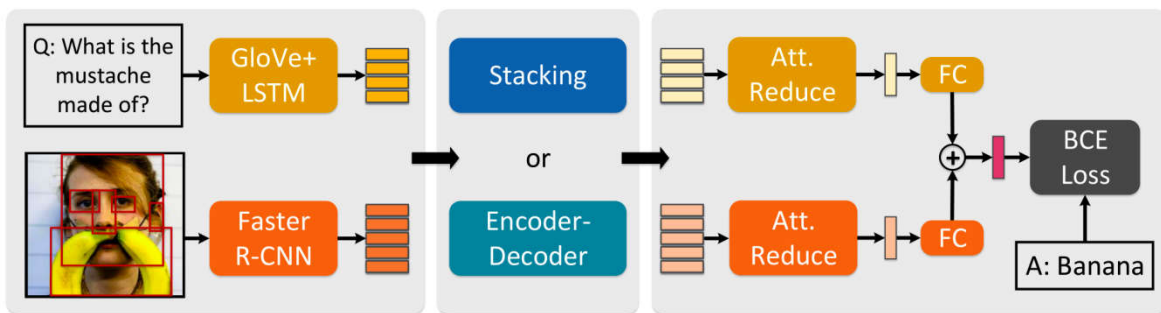
Fig.5 Overall flowchart of the deep Modular Co-Attention Networks [56]
