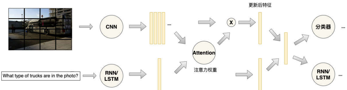
Fig.3 The framework of problem-guided attention methods
