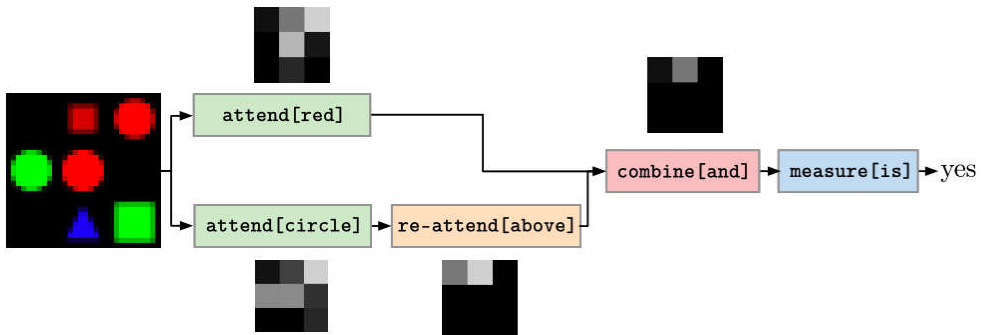
Fig.8 The overview of Neural Module Networks [64]
