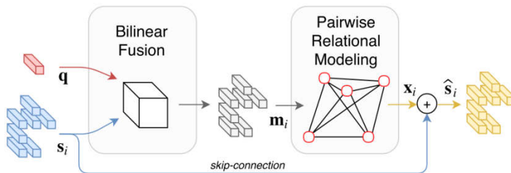
Fig.7 The overview of Murel cell [62]
