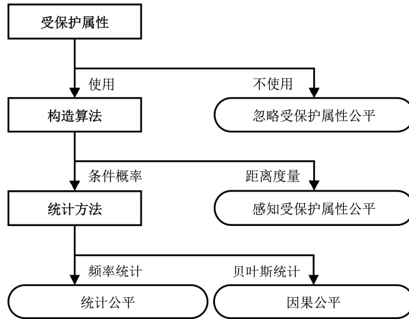
Fig.6 Fairness Definitions in Machine Learning
