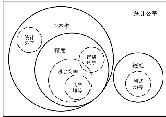
Fig.7 Relationship Between Statistical Fairness Definitions 图7 统计公平定义间的关系
