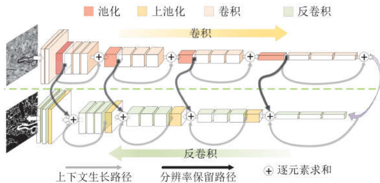
Fig.17 The RDN model for neuronal membrane segmentation
