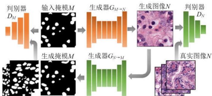
Fig.22 The CGAN-style architecture for nuclear segmentation
