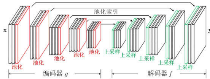
Fig.6 The architecture of a classical encoder-decoder model
