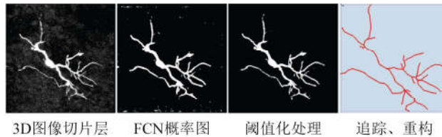
Fig.13 FCN based 3D neuron segmentation and reconstruction 图 13 基于 FCN 的三维神经元分割与重构
