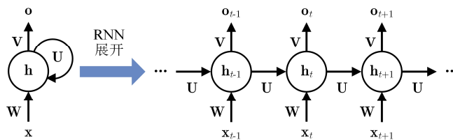
Fig.7 The schematic diagram of RNN
