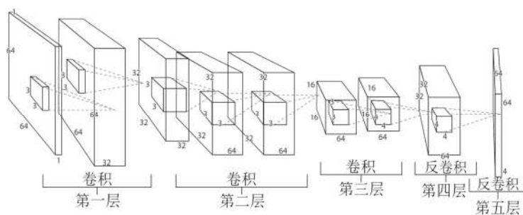
Fig.5 The architecture of FCN
