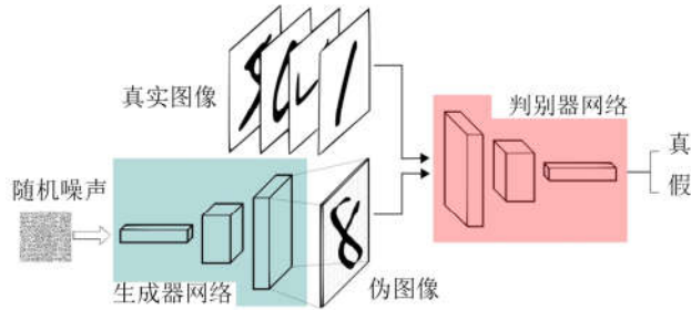
Fig.9 The architecture of GAN
