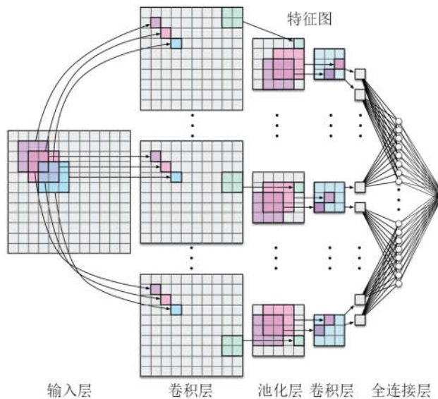
Fig.4 The architecture of CNN
