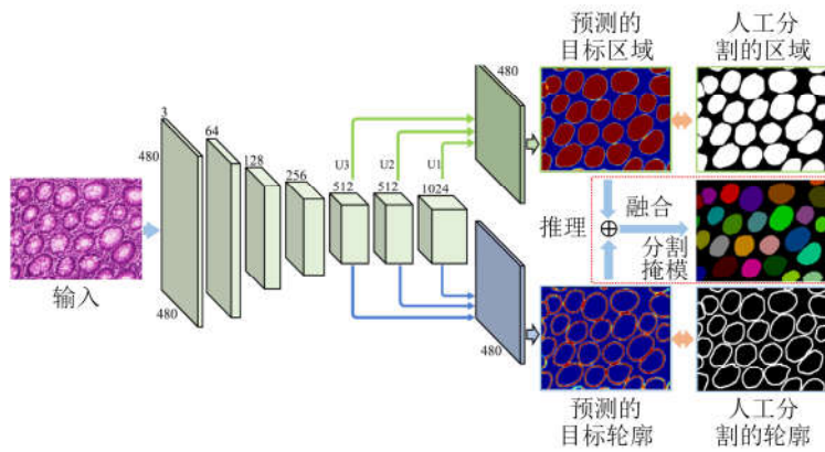
Fig.14 The DCAN model for gland and nucleus segmentation
