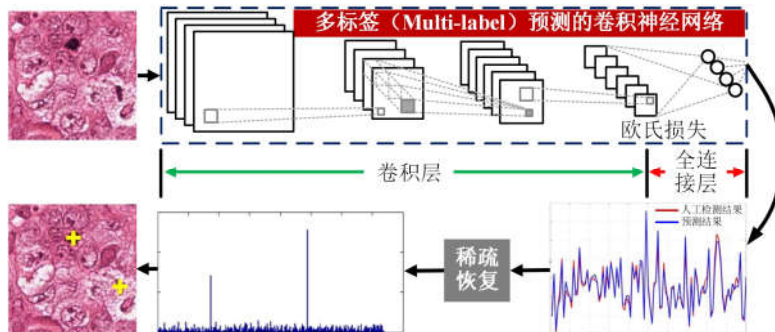
Fig.11 Cell detection by combining CNN and compressed sensing
