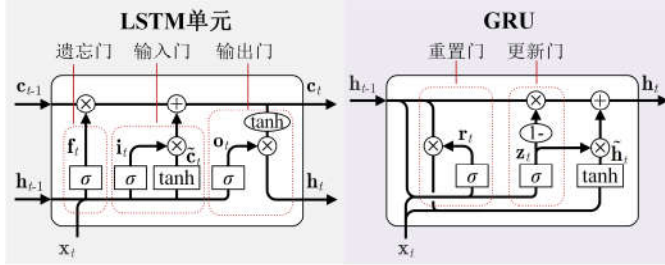
Fig.8 The structures of LSTM [62] and GRU [63] modules
