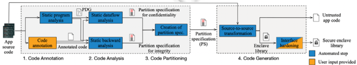
Fig.7 Overview of the Glamdring framework
