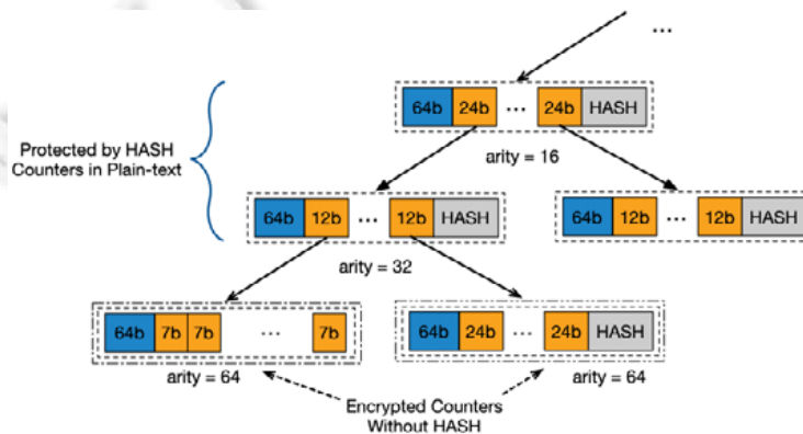
Fig.8 VAULT schematic diagram
