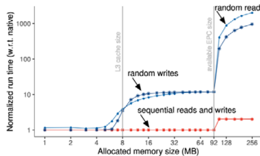
Fig.10 Normalized overhead of memory accesses with SGX enclaves
