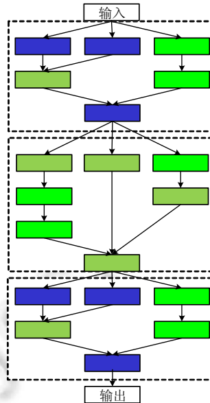
Fig.18 Neural network architecture based on block structure
