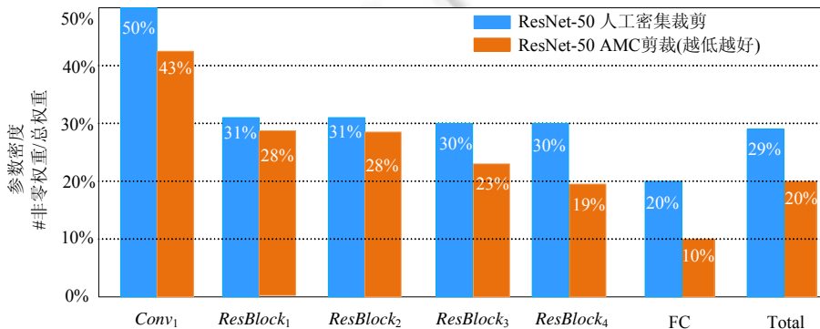
Fig. 13 Comparison between AMC and artificial design compression algorithm
