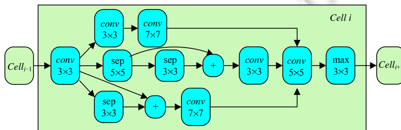
Fig.24 Neural network architecture search based on evolutionary algorithm
