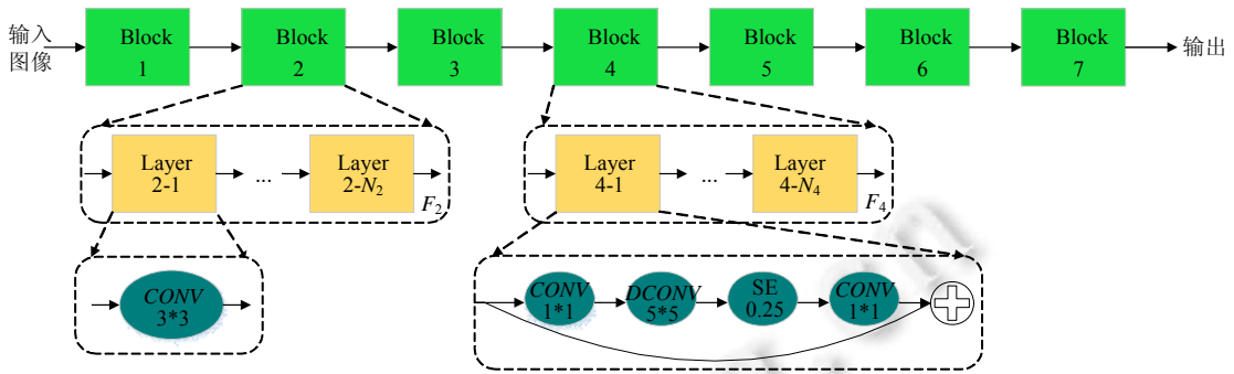
Fig.25 Decomposition of hierarchical search space
