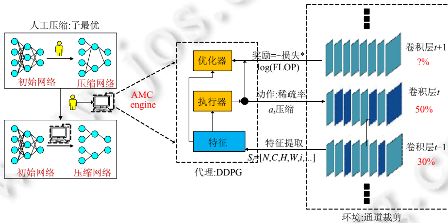
Fig. 12 The structure of AMC compression algorithm
