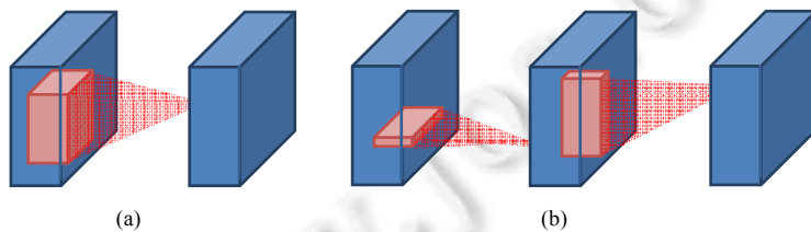
Fig.10 Low-rank decomposition of convolution kernels
