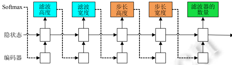
Fig.20 Autoregressive control structure
