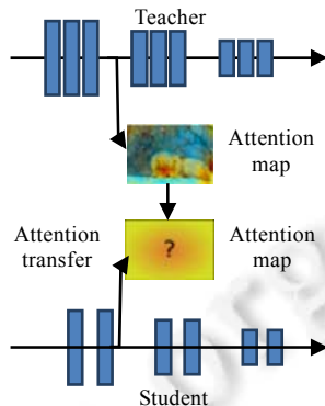
Fig.11 Knowledge distillation network (teacher-student network)
