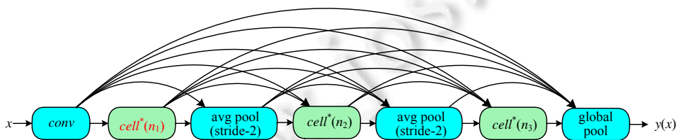
Fig.17 Densely connected mobile search space
