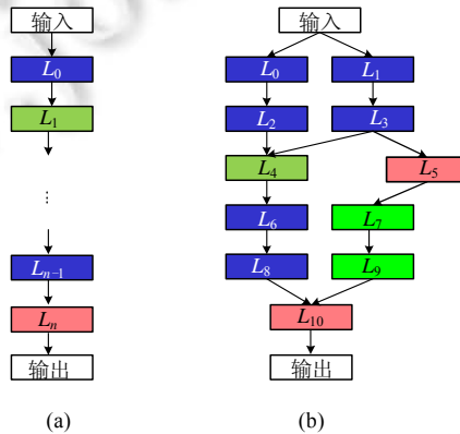
Fig.15 Chain and multi branch architecture search space
