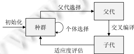
Fig.21 The framework of evolutionary algorithm
