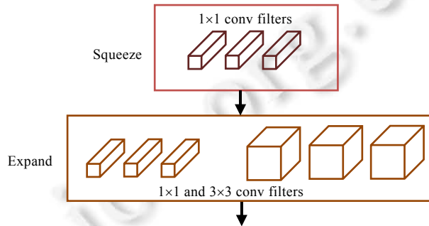
Fig.2 Organization of convolution filters in the Fire module. A Fire module is composed of a squeeze convolution layer and a expand layer
