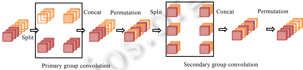
Fig.8 Organization of interleaved group convolutions V1
