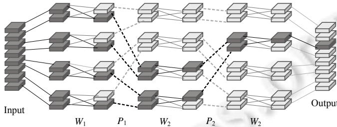
Fig.9 The interleaved structured sparse convolution (IGCV2) satisfying complementary condition
