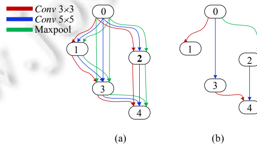
Fig.27 One-shot architecture search
