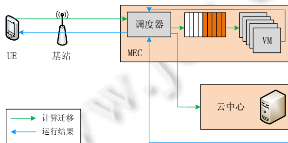
Fig.6 An example of MEC resource allocation
