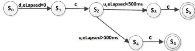
Fig.3 Click and LongClick event timed automata
