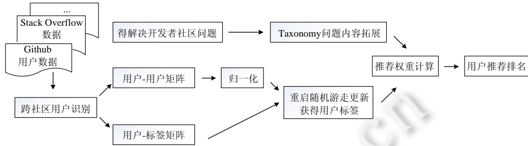
Fig.3 Algorithm framework
