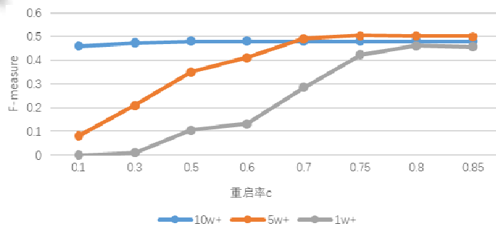
Fig.6 Different label area F-measure values under different restart rates
