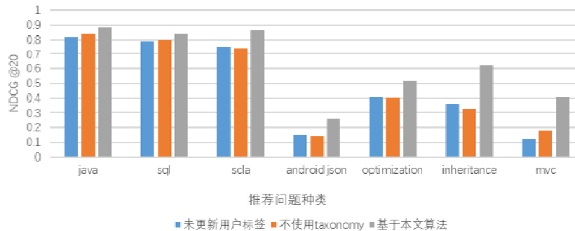
Fig.8 Do not consider the NDCG value under the user's ranking weight
