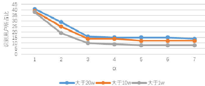
Fig.5 Different \alpha values and number of identified users in the label area
