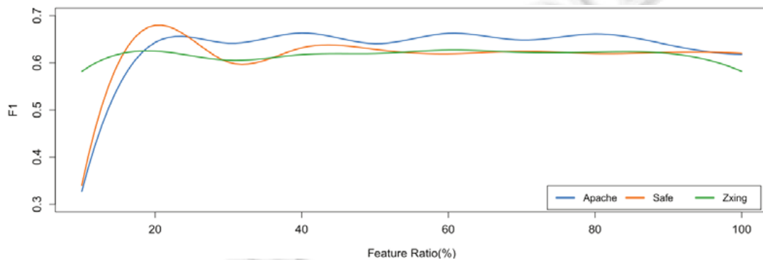
Fig.2 Impact on FeCTrA by varying feature transfer ratio on Relink
