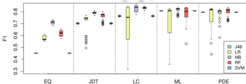
Fig.7 Impact on FeCTrA by using different basic classifier on AEEEM
