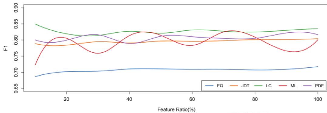
Fig.3 Impact on FeCTra by varying feature transfer ratio on AEEEM
