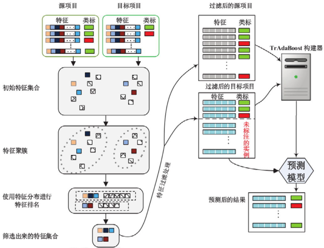
Fig.1 Cross-project software defect prediction framework based on feature transfer and instance transfer
