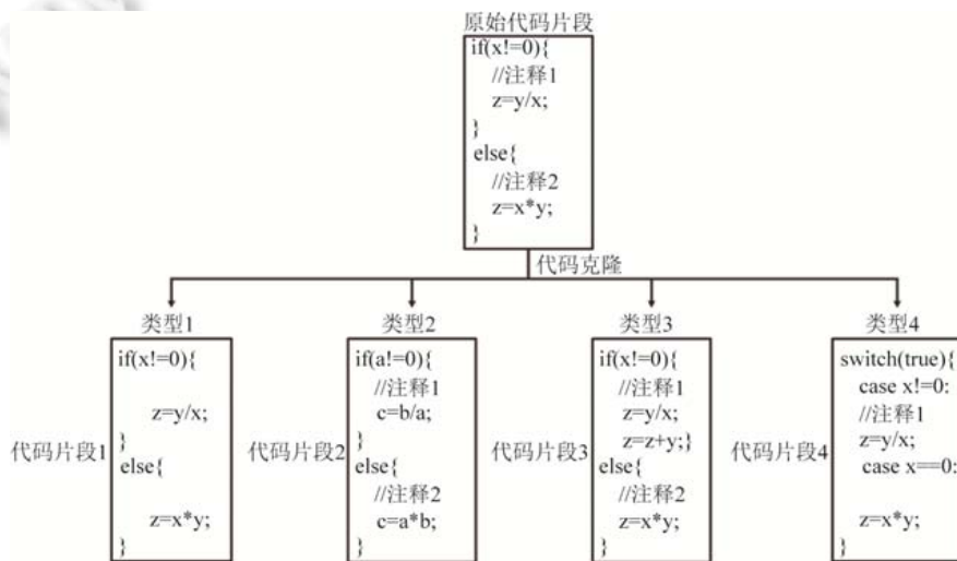
Fig.1 Original code fragment and four clone types
