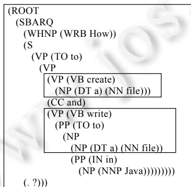
Fig.4 Natural language process for extracting action phrase (from StackOverflow question 2885173)
