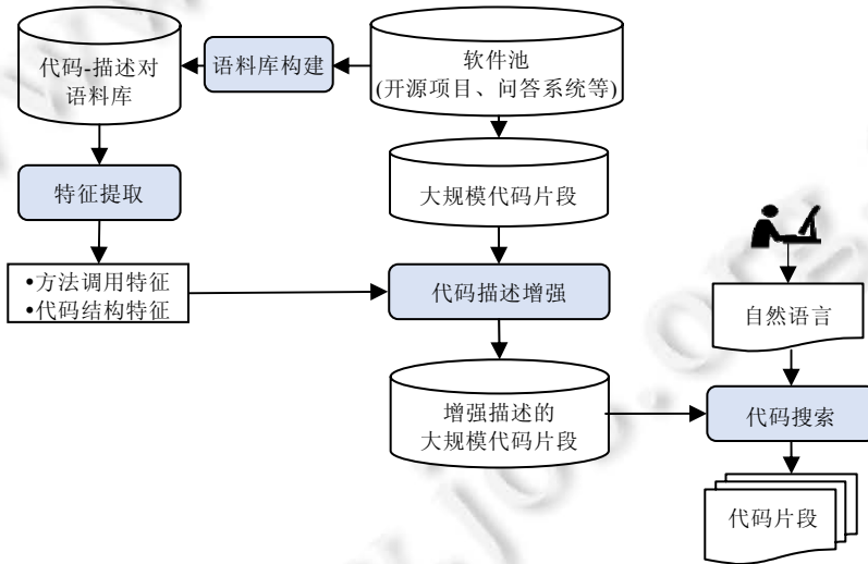
Fig.2 Approach overview of description reinforcement based code search
