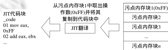
Fig.3 Operation of JIT translation
