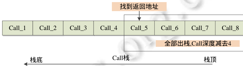
Fig.2 Operation of call stack
