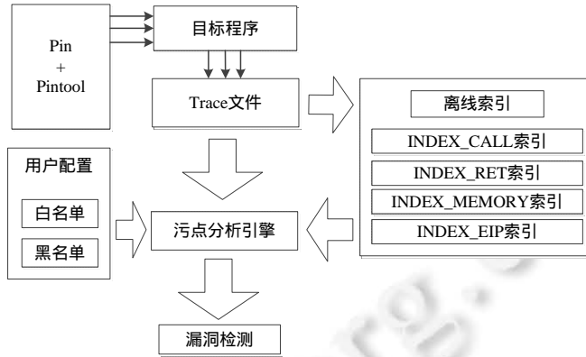
Fig.4 Structure of our system
