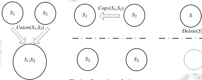
Fig.1 Operation of taint property
