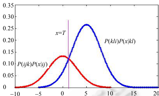
Fig.2 Optimal Bayes decision-making of subclass ij and kl
