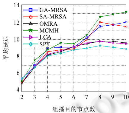
Fig.9 Average delay comparison (N=23)
