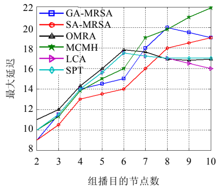
Fig.11 Maximum delay comparison ( N=23 )
