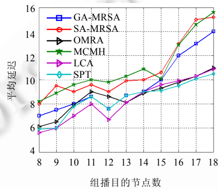
Fig.10 Average delay comparison (N=50)
