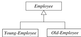
Fig.2 A fuzzy hierarchy relationship in a FOOD model
