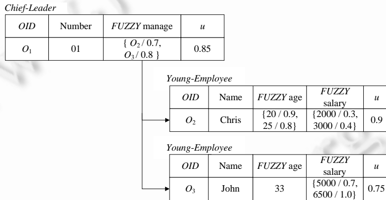
Fig.4 A fragment of a database instance w.r.t. the FOOD model FS_1 in Fig.3
