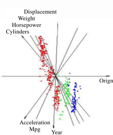
Fig.4 Visualization of cars using ASC
