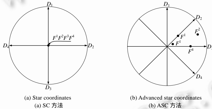
Fig.2 Comparison between ASC and SC
