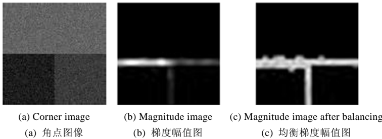
Fig.7 Magnitude balancing
