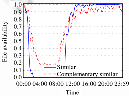
Fig. 12 The result of complementary similar on level 0.4
