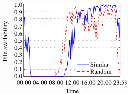
Fig.8 Comparison of availability on level 0.4
