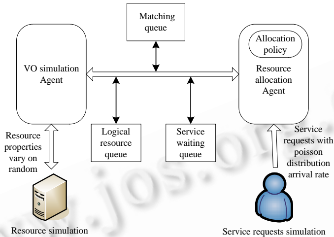
Fig.7 Simulated grid resource management system
