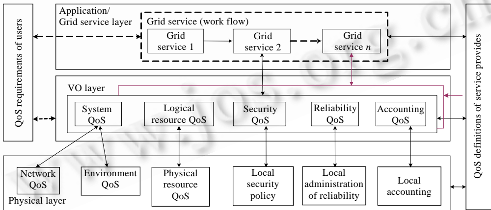
Fig.1 The hierarchical structure of grid QoS
