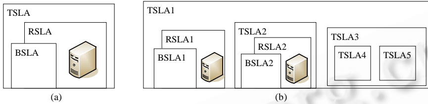
Fig.6 The composing relation between SLAs and grid service
