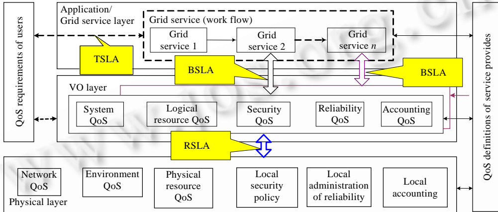
Fig.5 The relation between SLAs and QoS hierarchical structure
