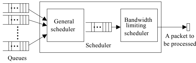
Fig.4 Architecture of the scheduler
