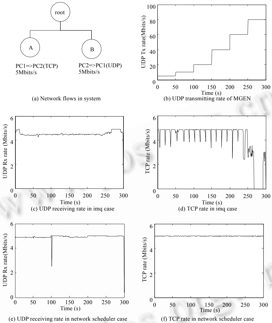
Fig.8 Traffic isolation test configuration and results
