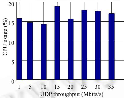
(a) CPU usage of Linux with IMQ enabled TC
