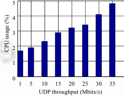
(b) CPU usage of Linux with network scheduler
