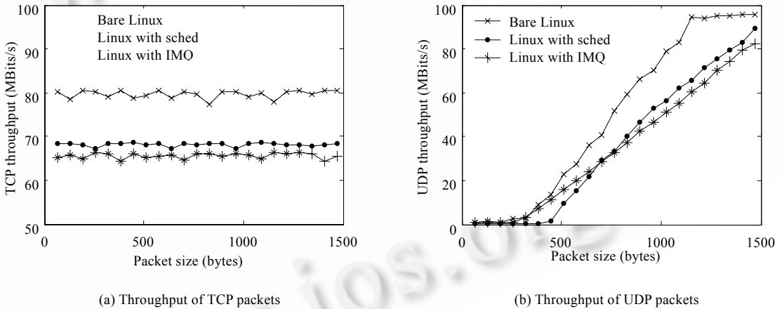
Fig.6 Throughput statistics for different IP packet sizes
