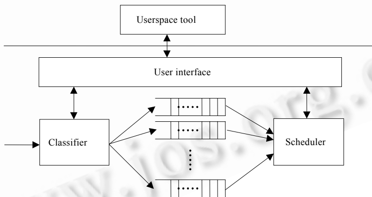
Fig.2 Architecture of new traffic control mechanism
