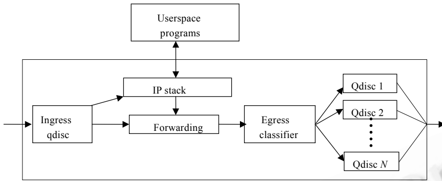
Fig.1 Architecture of Linux traffic control
