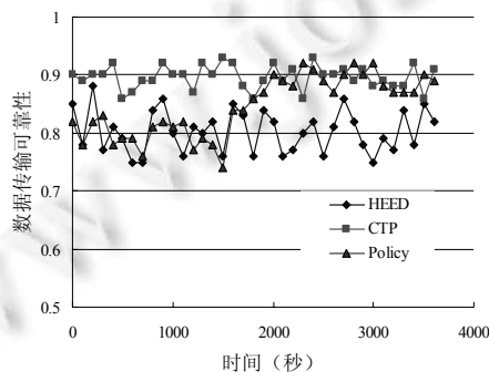
Fig. 12 End-to-End reliability of data transmission
