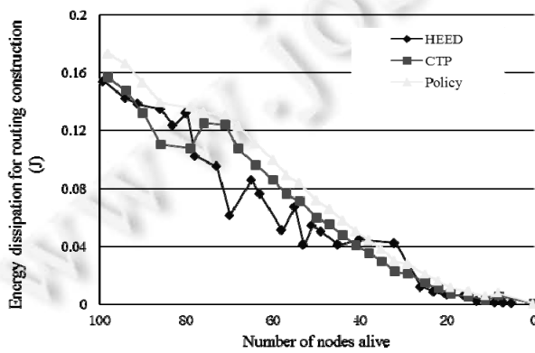
Fig.15 Energy costs of routing protocols 图 15 路由的建立和维护的能量开销
