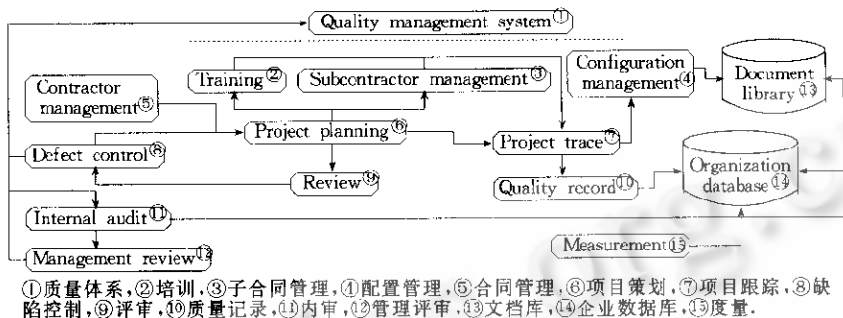
Fig.1 The relationship between the processes of software quality management model based ISO9000 & CMM 图1 基于ISO9000和CMM的软件质量管理模型各过程之间的关系
