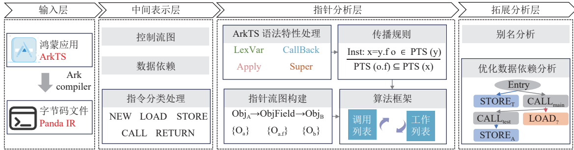
图2 HarmonyFlow 框架设计概览
