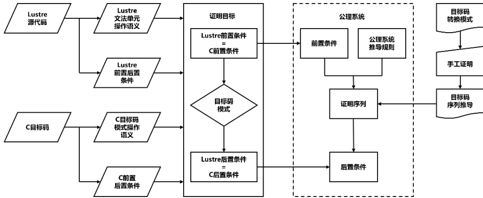
Fig.5 Formal Verification System Architecture Diagram
