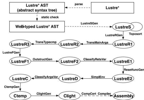
Fig.2 Translation Process of the L2C Compiler
