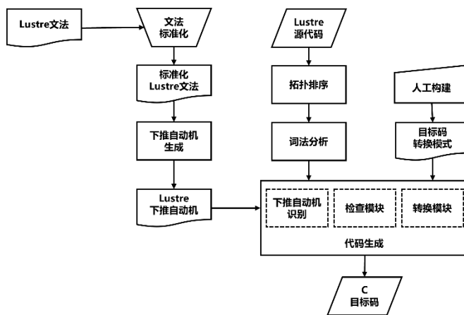
Fig.3 Compilation System Architecture Diagram
