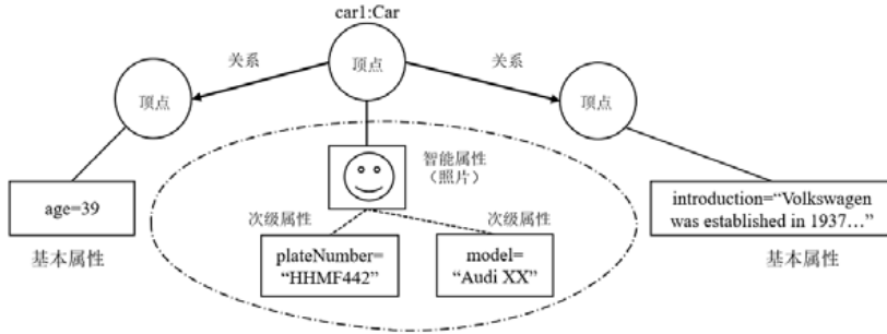
Fig.1 Intelligent property graph model
