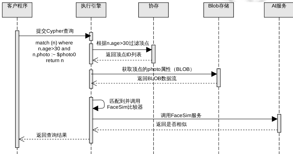
Fig.7 CypherPlus query process
