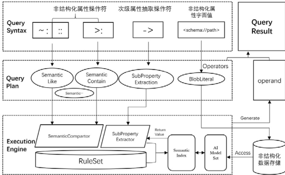
Fig.8 Query mechanism of intelligent property graph 图 8 智能属性图查询机制
