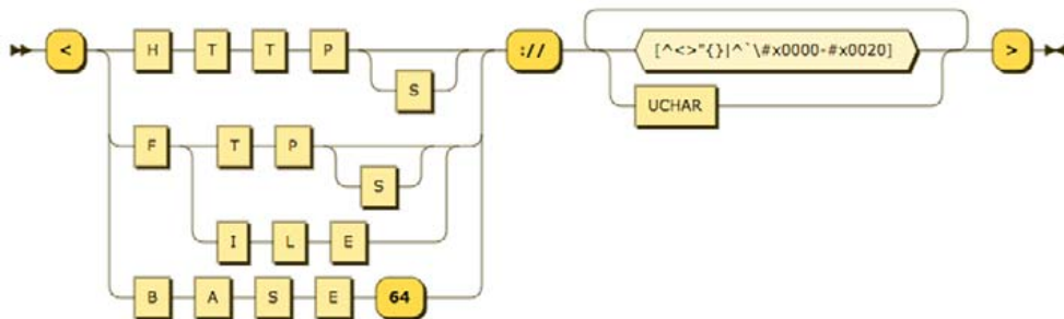
Fig.2 Grammer definition of BlobLiteral
