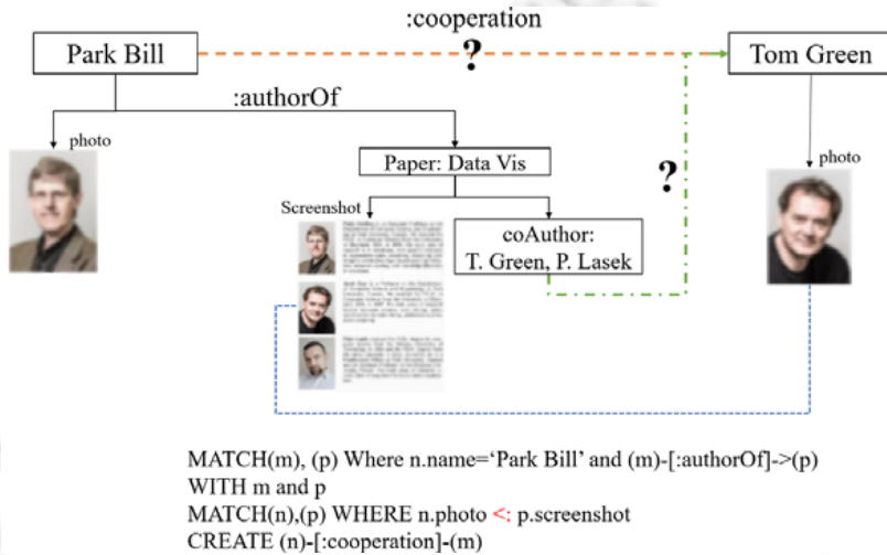
Fig.15 Diagram of entity disambiguation based on PandaDB
