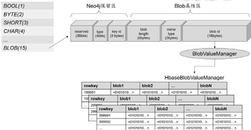
Fig.6 Design of BLOB storage structure
