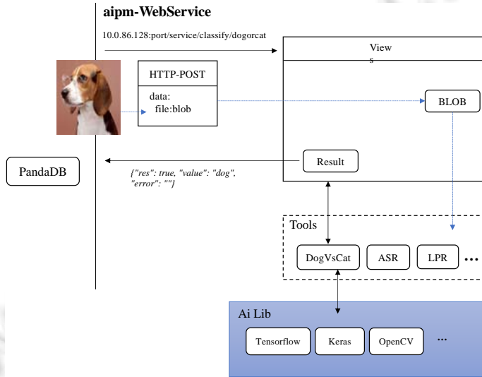
Fig.11 Interaction of PandaDB and AIPM
