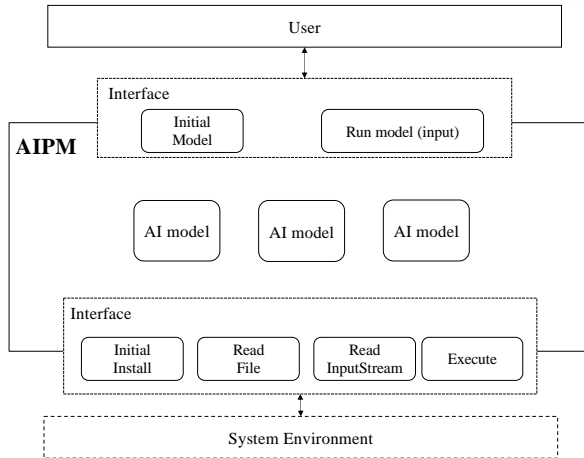
Fig.12 AI model management framework
