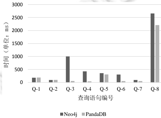
Fig. 13 Comparison of query time in co-store
