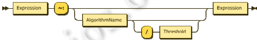
Fig.4 Grammer definition of SemanticLike
