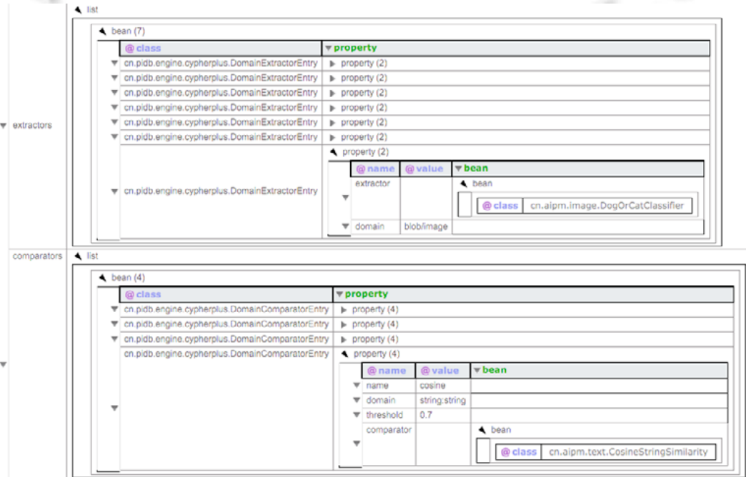
Fig.10 Extractor and semantic comparator matching rule set
