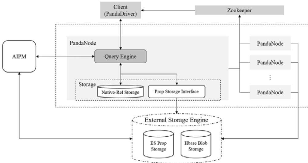
Fig.5 Architecture of PandaDB
