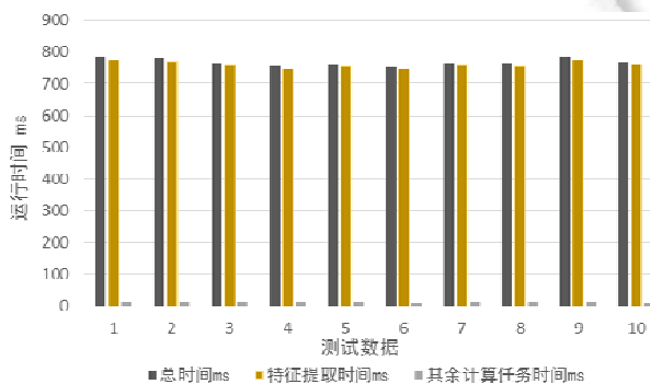
Fig.8 Terminal node calculation task processing time (calculation task completely local calculation)
