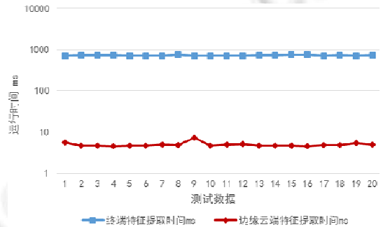
Fig.12 Feature extraction time comparison chart offloading strategy of neural network model
