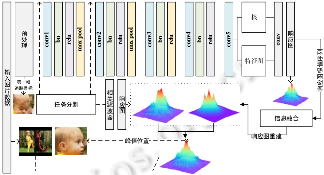
Fig.5 Schematic diagram of the calculation process of the task (picture is OTB100 [29] DragonBaby)
