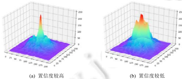
Fig.6 Filter response map
