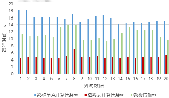
Fig.11 Computing task processing time in complete
