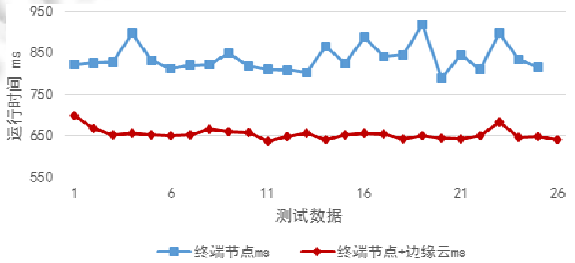
Fig.16 Track task overall calculation time 图 16 追踪任务总体计算时间
