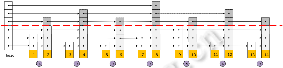
Fig.7 Example of partition-based skiplist
