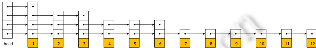
Fig.2 Example of skiplist in worst case
