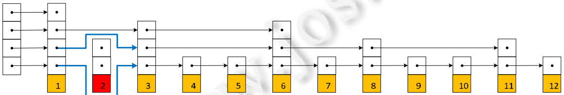
Fig.5 Example of delete node 2 in skip list 图 5 删除结点 2 的示例
