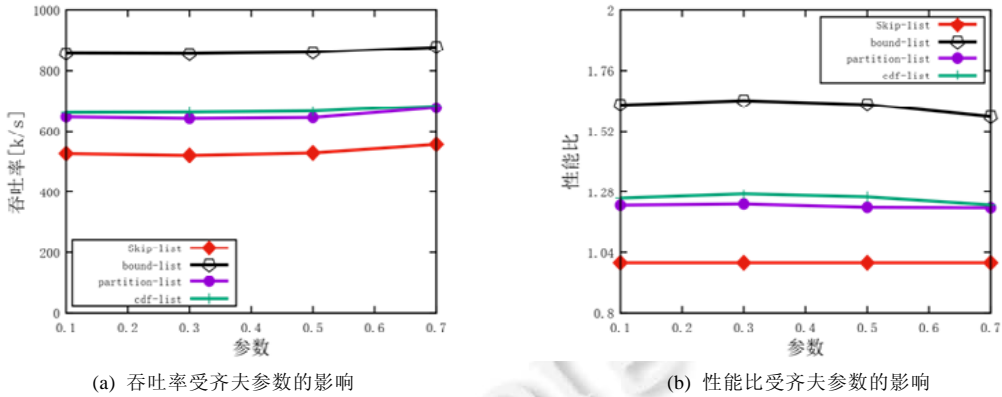
Fig.9 Performance influenced by the parameter of Zipfian distribution
