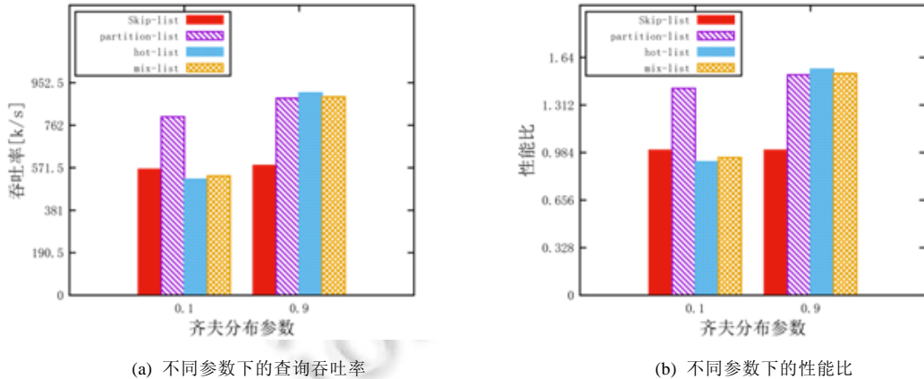
Fig.16 Performance under different Zipfian distribution dataset
