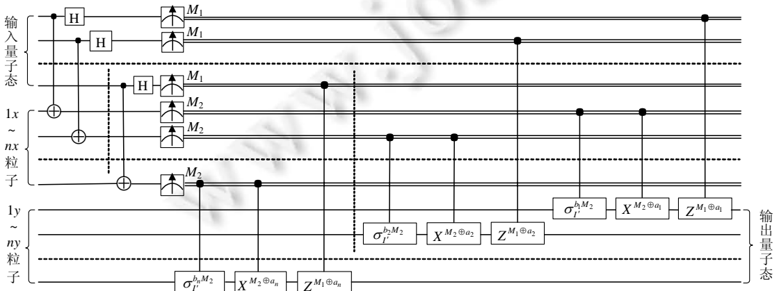
Fig.8 Universal circuit for N-qubit quantum teleportation
