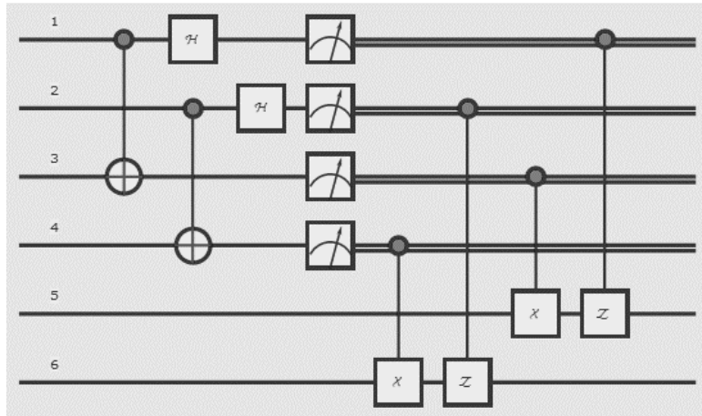
Fig.6 Two-qubit quantum teleportation
