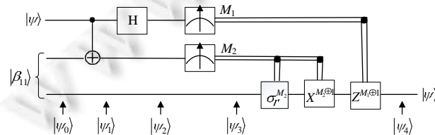
Fig.4 Quantum teleportation for |\beta_{11}\rangle
