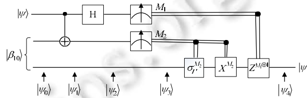
Fig.3 Quantum teleportation for |\beta_{10}\rangle
