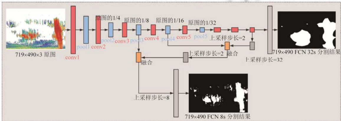
Fig.3 The framework of FCN
