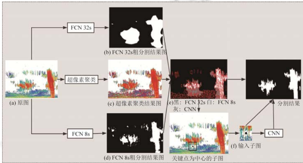
Fig.2 An overview of the proposed FCN-CNN for cloud image segmentation
