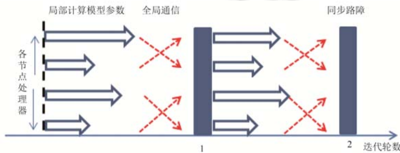
Fig.2 Bulk synchronous parallel model
