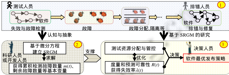
Fig.2 Modeling flow and function of the SRGM
