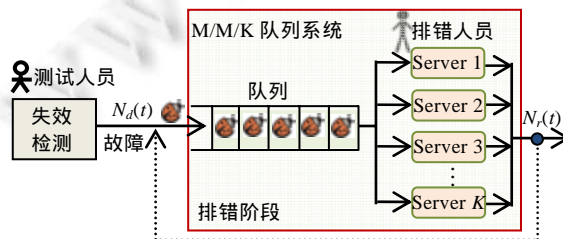
Fig.5 Software debugging queue: A single-queue multichannel debugging queuing system
