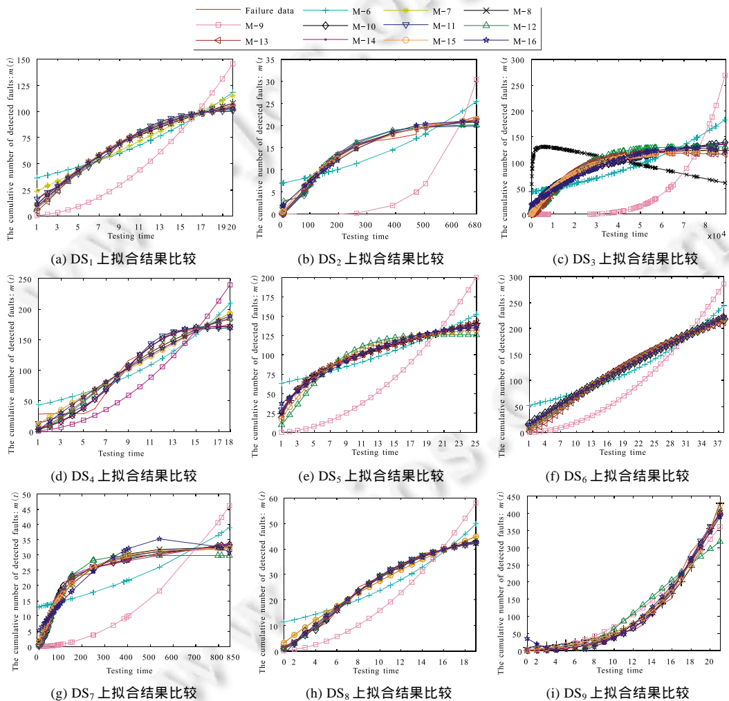
Fig.8 Fitting curves of M-6 to M-16 on DS 1 ~DS 9
