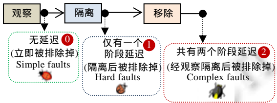
Fig.6 Simple, hard and complex faults 图 6 简单、严重和复杂这三种故障类型
