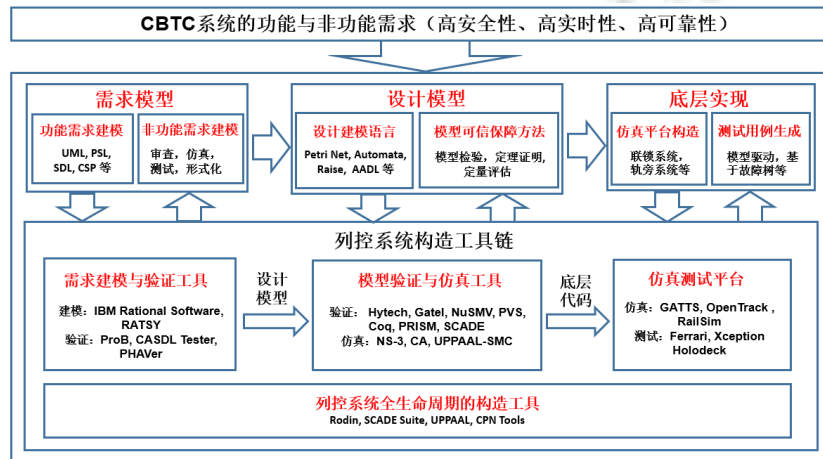
Fig.1 Trustworthy construction framework for CBTC based on formal methods
