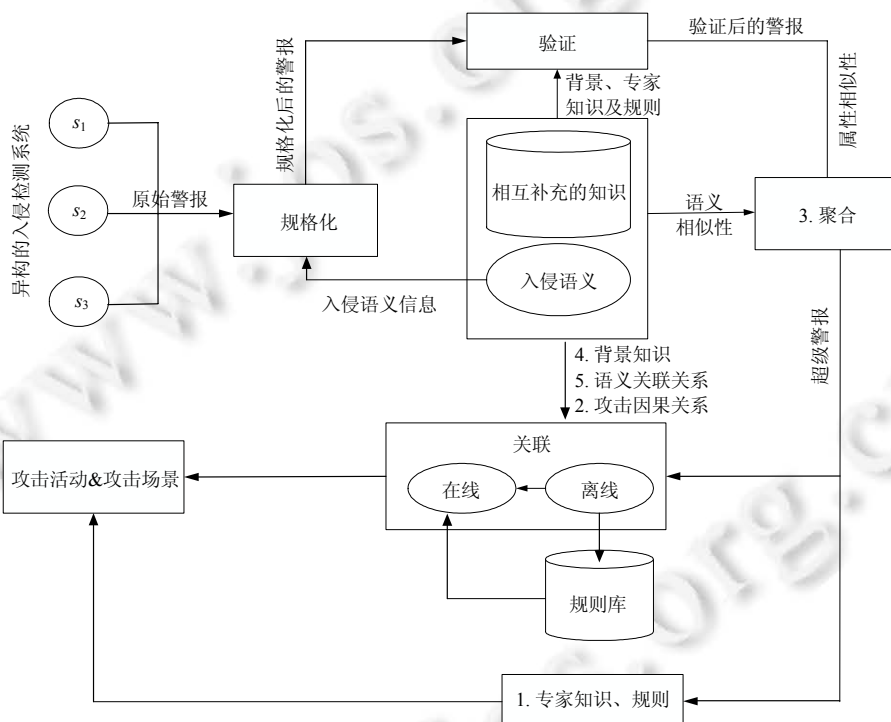
Fig.5 Attack activities reconstruction model
