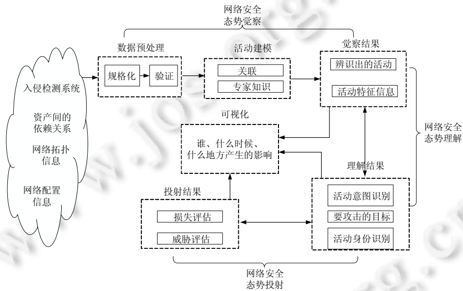
Fig.3 Network situation awareness model
