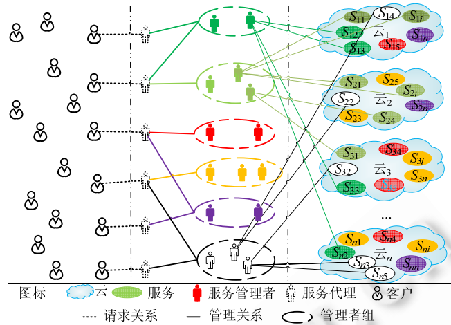
Fig.1 Self-Organizing management model of cloud services based on multi-agent system
