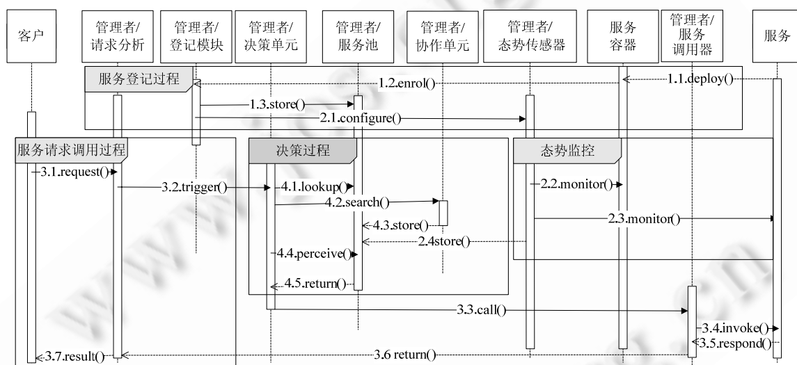
Fig.6 Autonomous management process of self-organizing management entity
