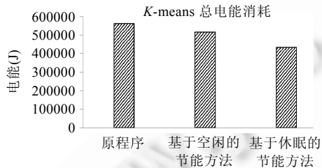
Fig.19 Total energy consumption of k -means
