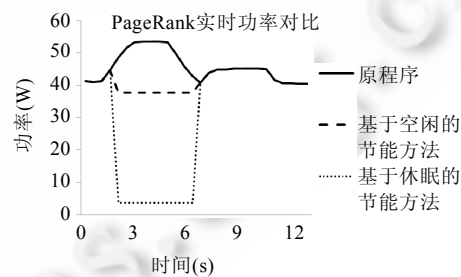
Fig.16 Realtime power of PageRank
