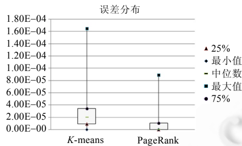
Fig.21 Error distribution of PageRank and k -means
