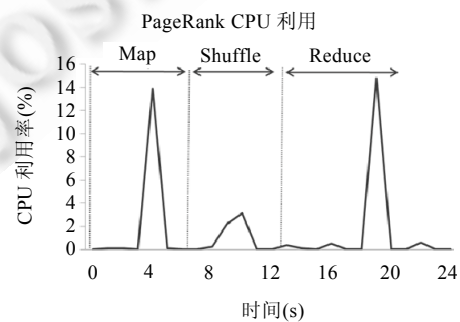
Fig.2 CPU usage (PageRank)
