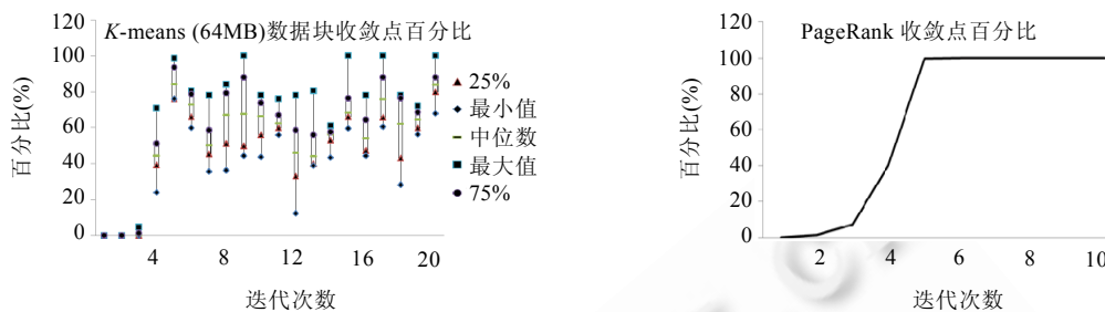
Fig.7 Percentage of converged points in k -means (64MB) Fig.8 Percentage of converged points in PageRank
