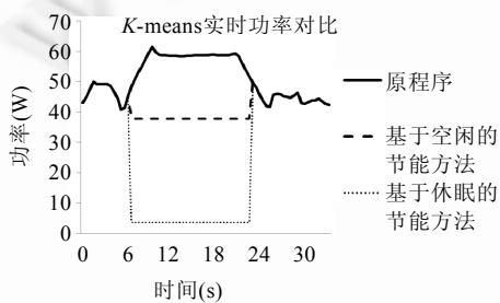
Fig.15 Realtime power of k -means
