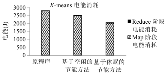
Fig.17 Energy consumption of k -means
