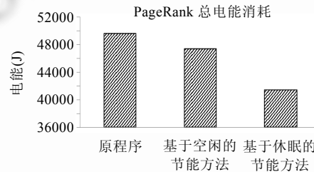
Fig.20 Total energy consumption of PageRank
