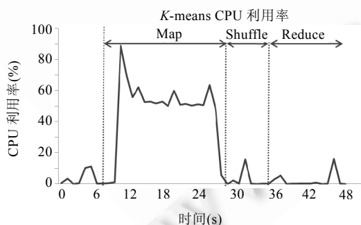
Fig.1 CPU usage (K-means)
