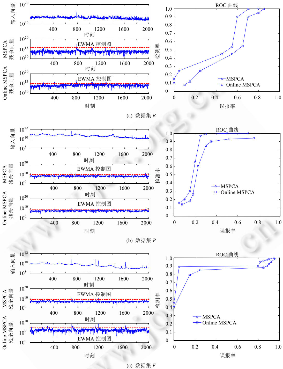
Fig.4 Detection result and performance of MSPCA and online MSPCA algorithm for real measurement data
