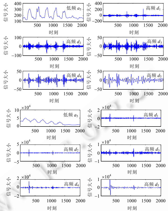
Fig.14 Low frequency and high frequency components of OD1 (up) and OD121 (down) traffic signal
