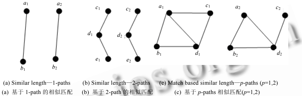
Fig.5 p -path local match rule [34]
