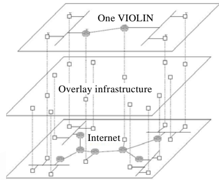
Fig.2 VIOLIN architecture 图 2 VIOLIN 体系结构
