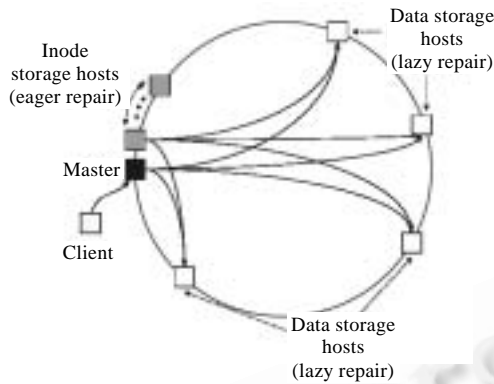
Fig.10 Architecture of Total Recall 图 10 Total Recall 的系统结构
