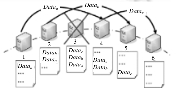
Fig.11 Data repair in sequential placement
