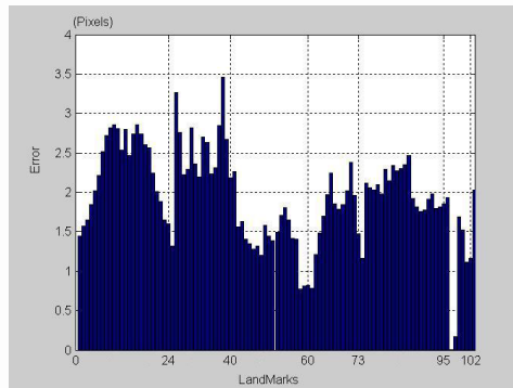
Fig.4 The error distribution of the distance from the automatic landmarks label results to the ground-truth 图 4 特征点自动标定结果与手工标定点距离的误差分布
