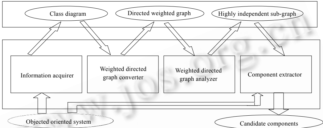
Fig.4 A candidate component extraction system based on analysis of the directed weighted graph
