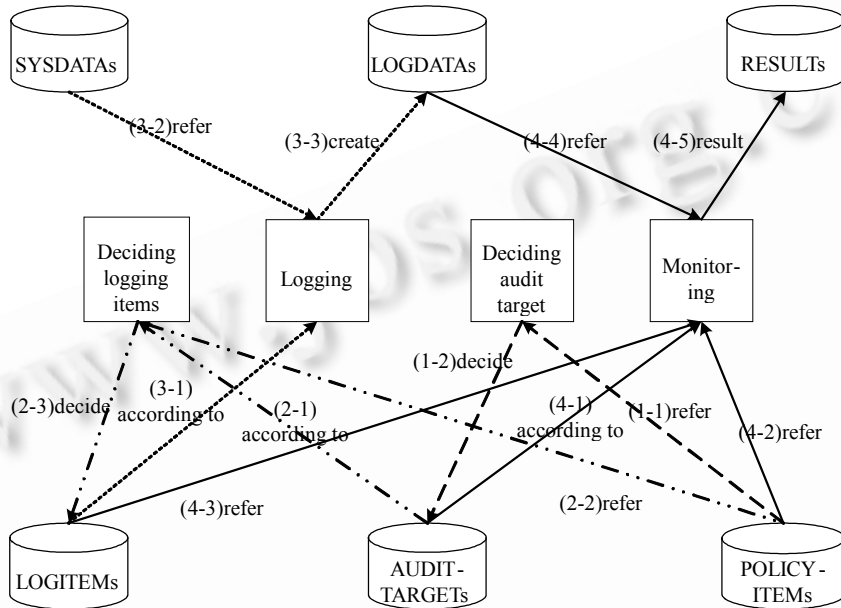
Fig.2 Illustration of secure monitoring model
