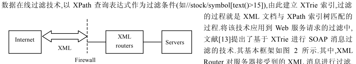
Fig.2 The system architecture of SOAP message filtering 图2 SOSAP 消息过滤系统架构
