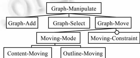
Fig.1 DFM fragment of graph editor
