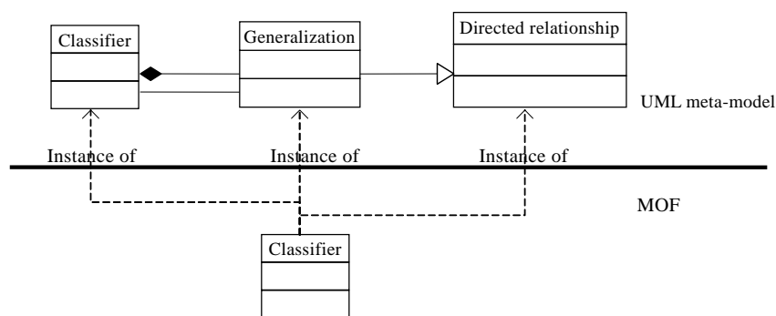
Fig.2 UML relationship and MOF classifier
