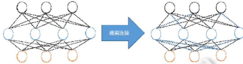
Fig.3 Pruning connections
