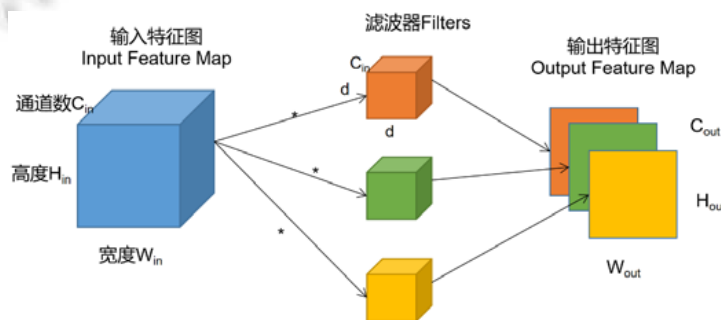
Fig.1 Convolutional operator
