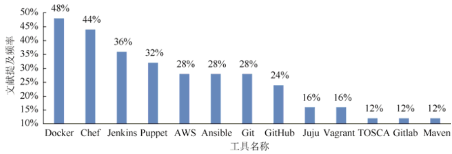
Fig.4 Frequency of automation tools in support of DevOps in studies
