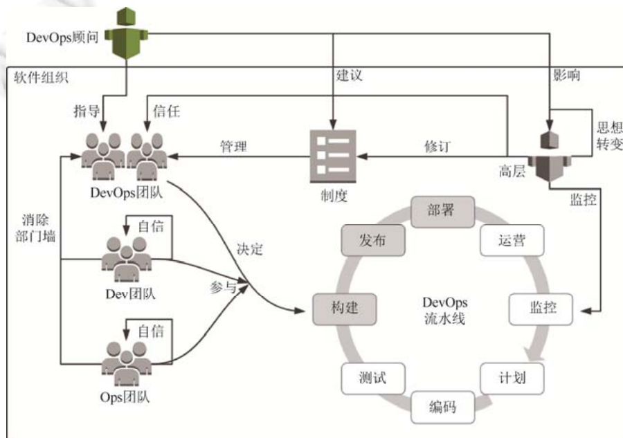
Fig.10 DevOps paradigm for software organization
