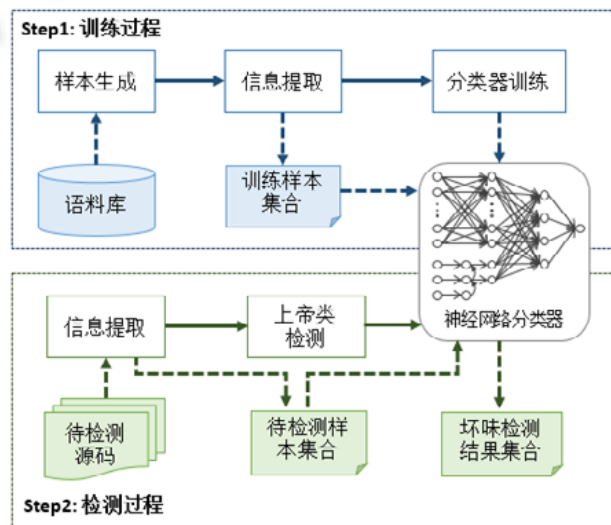
Fig.1 Overview of the god class detection based on deep learning
