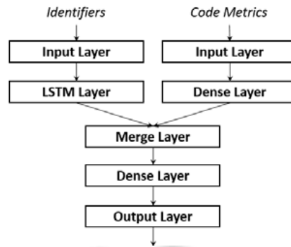
Fig.2 Classifier based on neural network
