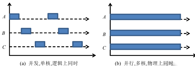
Fig.1 The difference between concurrency and parallelism
