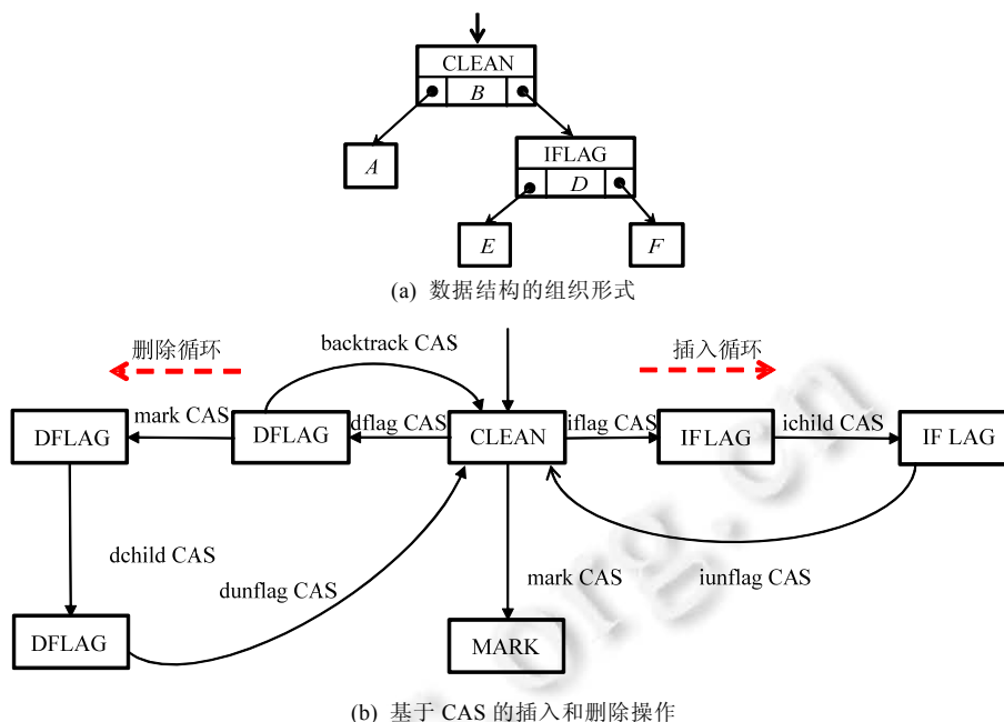
Fig.7 The diagram of the flag and atomic operations
