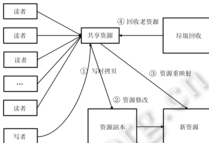
Fig.6 The RCU running mechanism
