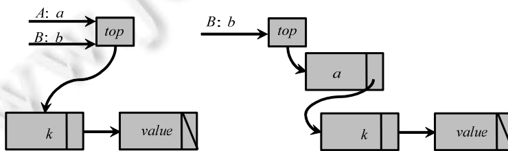
Fig.4 The concurrent stack implementation
